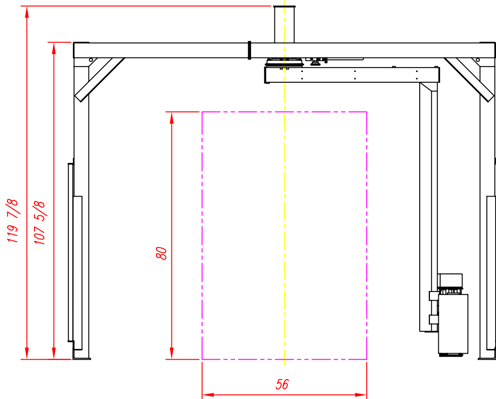
PRTG-2200 SEMI-AUTO ROTARY ARM GANTRY
